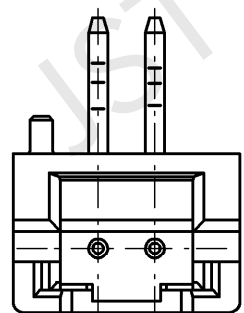
2極形状 Configuration of 2-circuit
