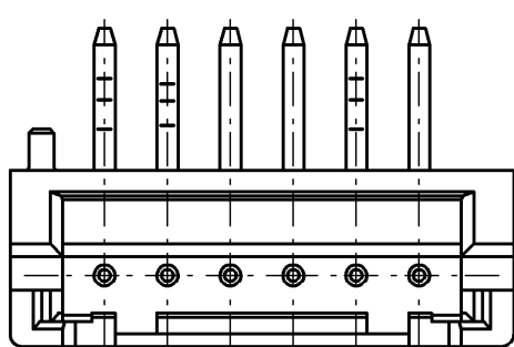
3~6極形状 Configuration of 3 to 6-circuit
