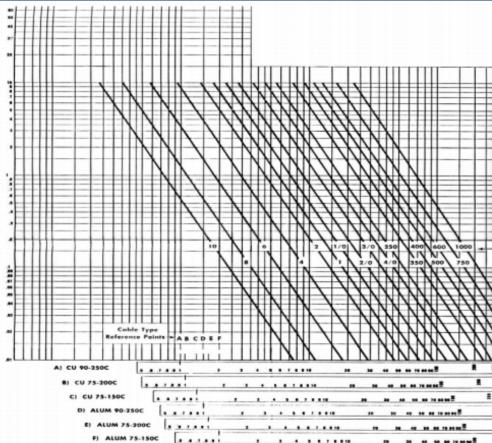
CURRENT IN TOTAL RMS KILOAMPS INSULATED CABLE SHORT CIRCUIT HEATING LIMITS
