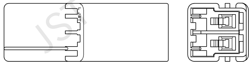
2極形状 Configuration of 2-circuits
