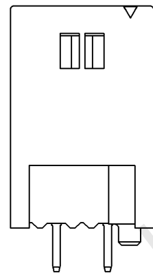
4極形状 Configuration of 4-circuits
