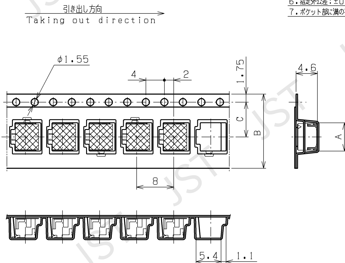
2~4極の形状 For 2 to 4 circuits connector.
