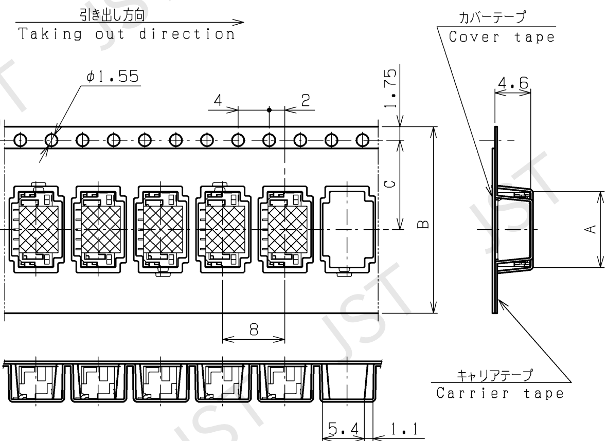
5極の形状 For 5 circuits connector.
