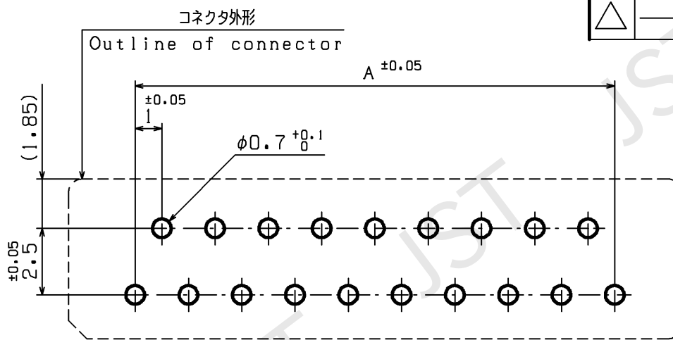
推奨基板穴寸法 (コネクタ装着側) Recommendable P.C.Board hole layout (Connector mounted side)
