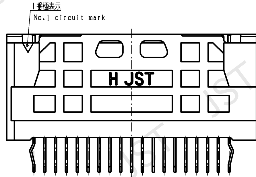
13~19極形状 Configuration of 13 to 19-circuit
