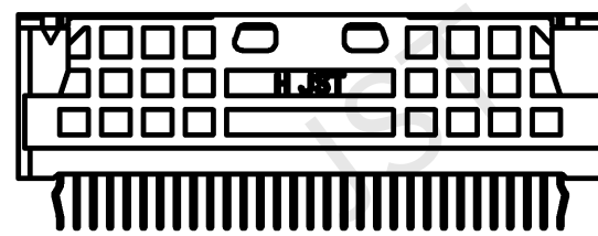
21~31極形状 Configuration of 21 to 31-circuit
