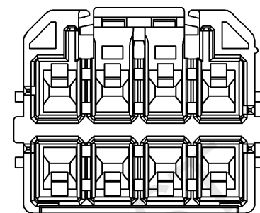
8極形状 Configuration of 8-circuits
