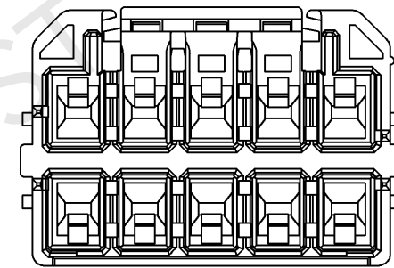
10極形状 Configuration of 10-circuits
