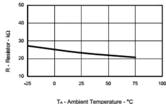
RESISTOR vs. AMBIENT TEMPERATURE
