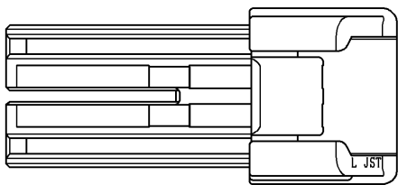
4極形状 Configuration of 4-circuits
