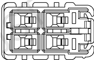
4極形状 Configuration of 4-circuits
