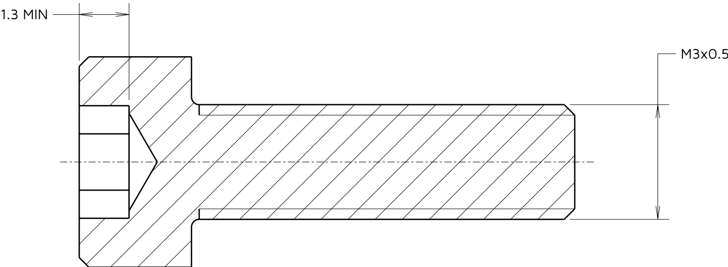
SECTION X-X
