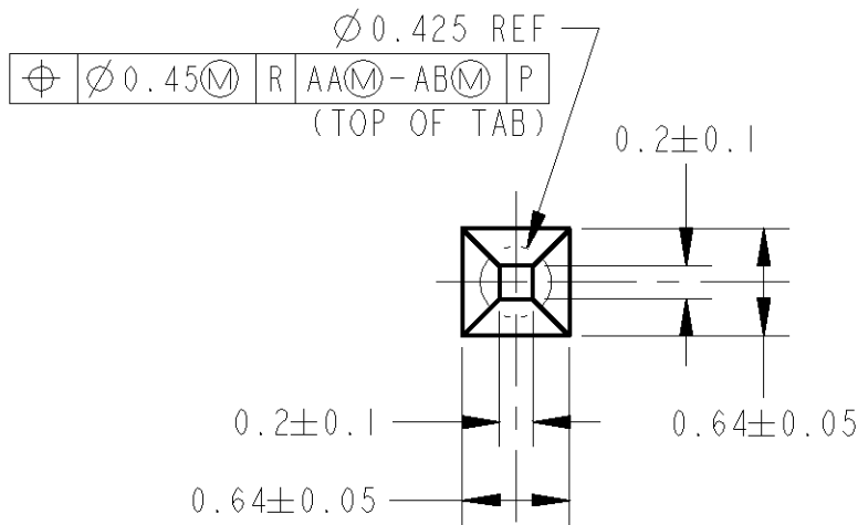
DETAIL C SCALE 20:1
