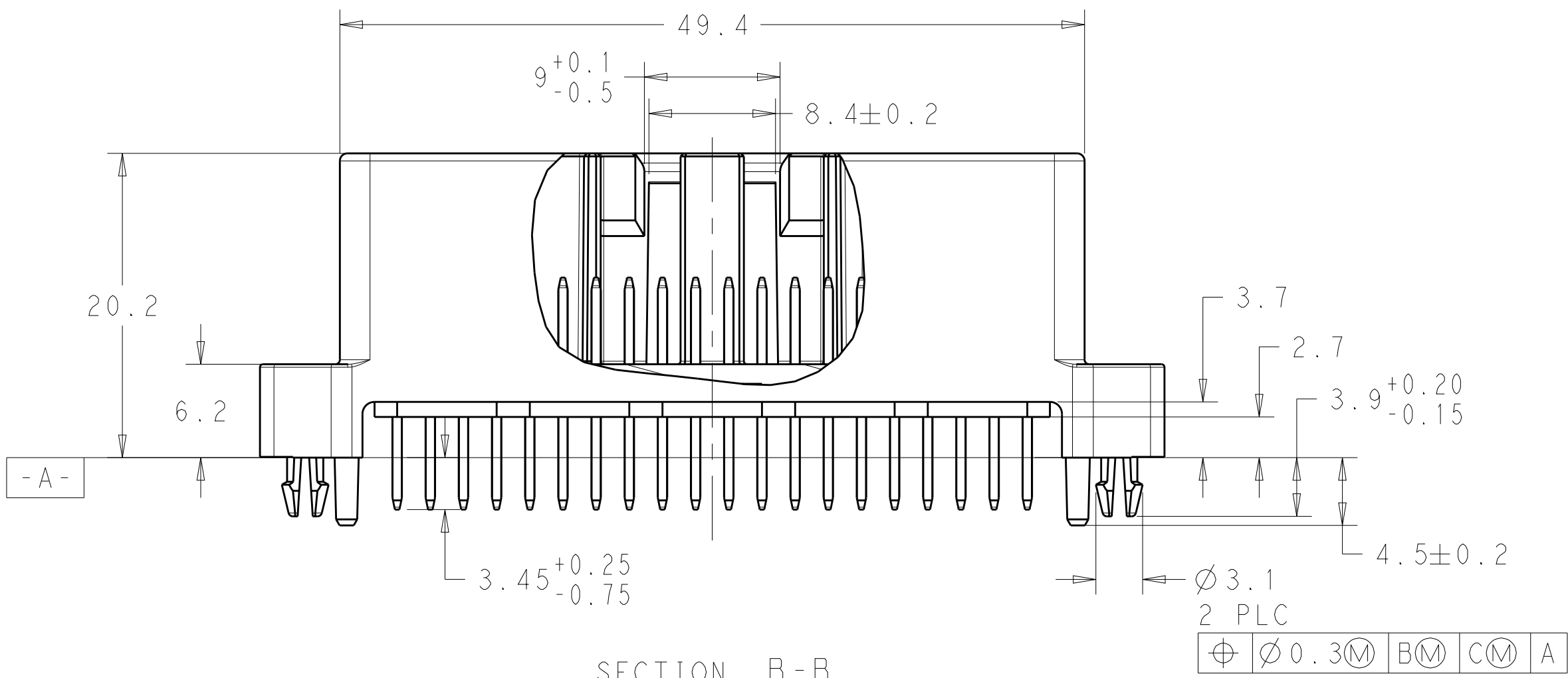
SECTION B-B
