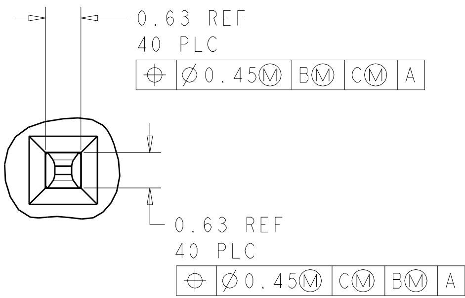
DETAIL MQS SCALE 15:1
