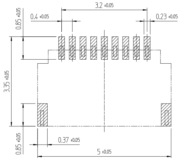
RECOMMENDED PCB MOUNTING PATTERN (Non scale) (RCOMMENDED METAL MASK THICKNESS : t=0.10)
