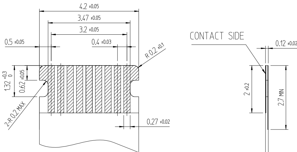
RECOMMENDED FPC (10:1)
