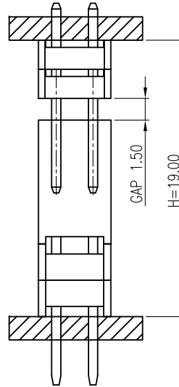
MATING VIEW
