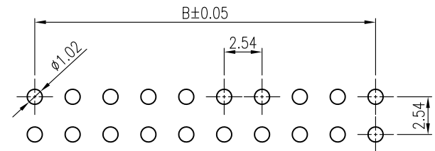
RECOMMENDED PCB LAYOUT ALL TOLERANCE ±0.05
