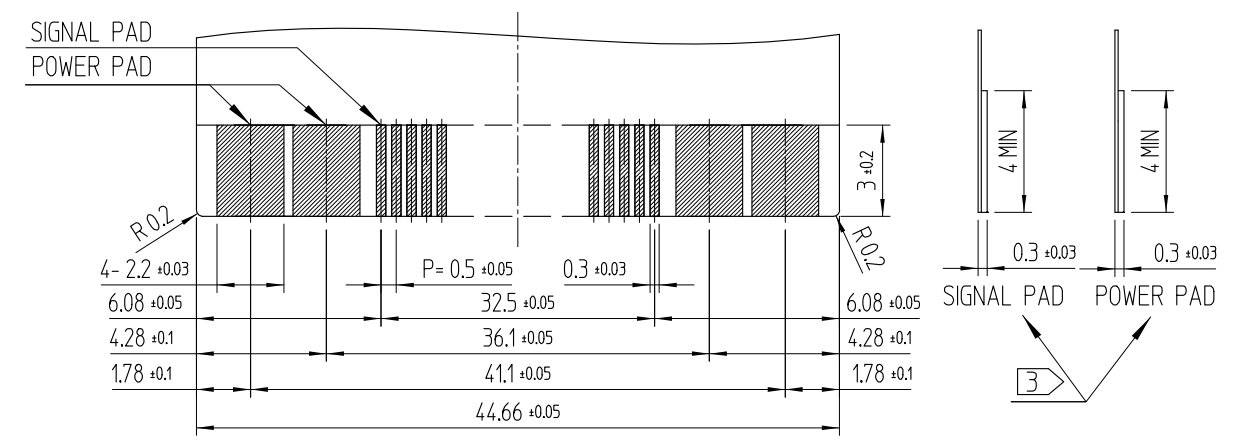
RECOMMENDED FPC/FFC(No scale)
