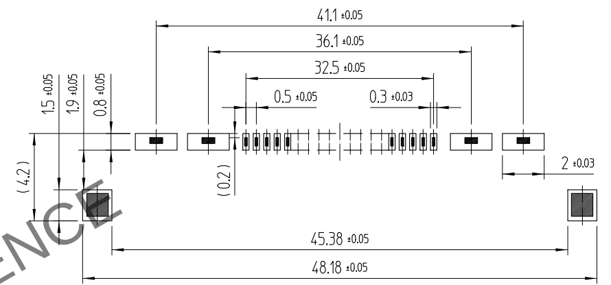
RECOMMENDED LAND PATTERN , METAL MASK (No Scale) RECOMMENDED METAL MASK THICKNESS : t=0.12
