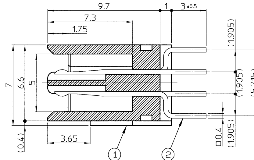
X-X' Cross-section(Scale 5:1)
