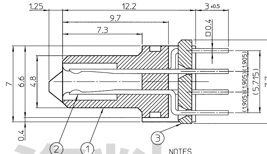
X-X' Cross-section(Scale 5:1)
