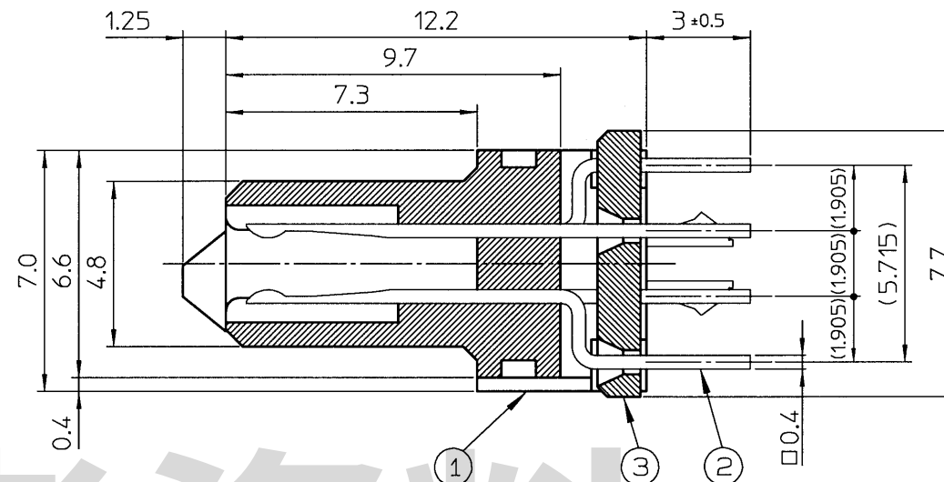
X-X' Cross-section (Scale 5:1)
