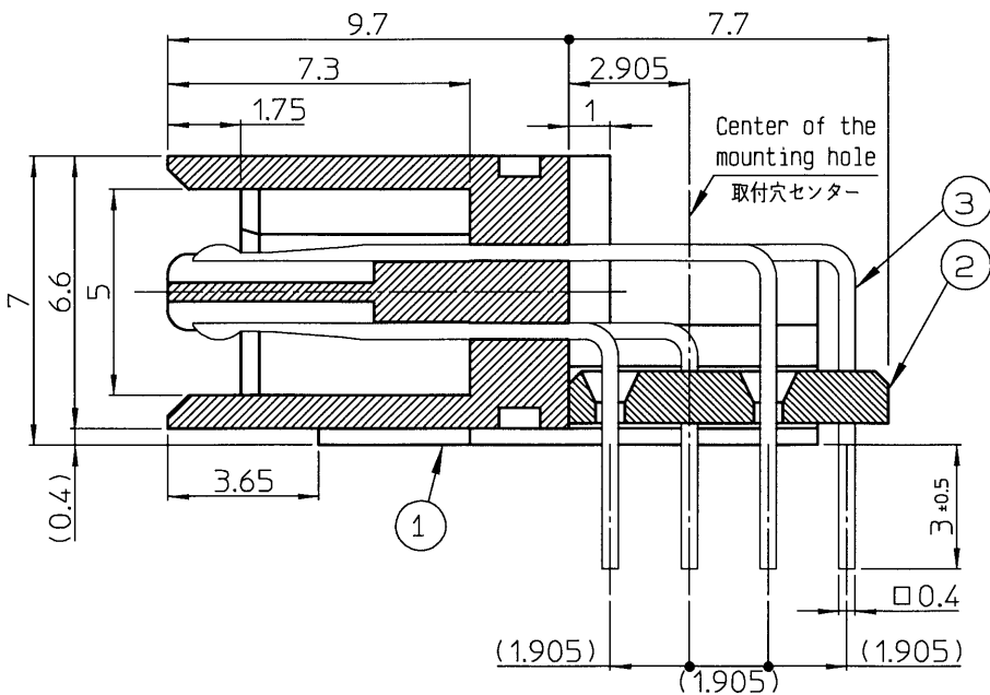
X-X' Cross-section(Scale 5:1)
