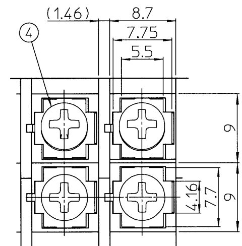
A section (Scale 2:1) Spring lock washers/セムスネジ(バネ座金付き)
