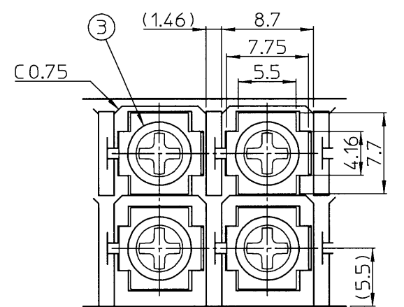
A section (Scale 2:1) Spring lock washers/セムスネジ(バネ座金付き)
