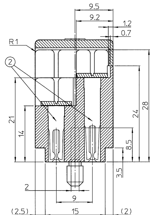
X-X' Cross-section (Scale 2:1)
