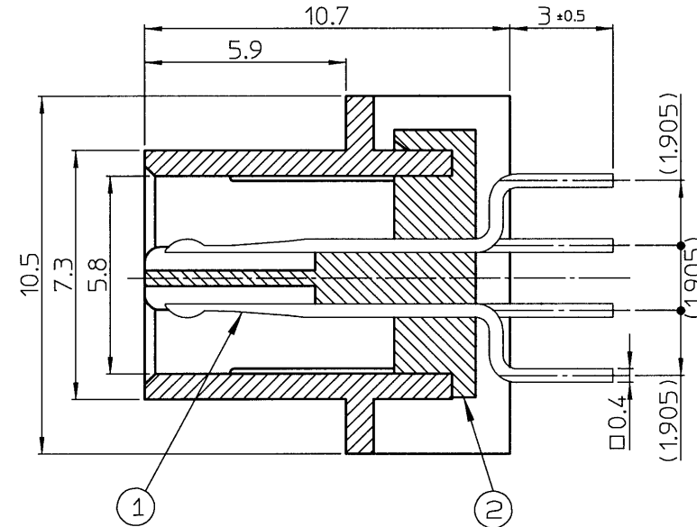
X-X' Cross-section (Scale 5:1)
