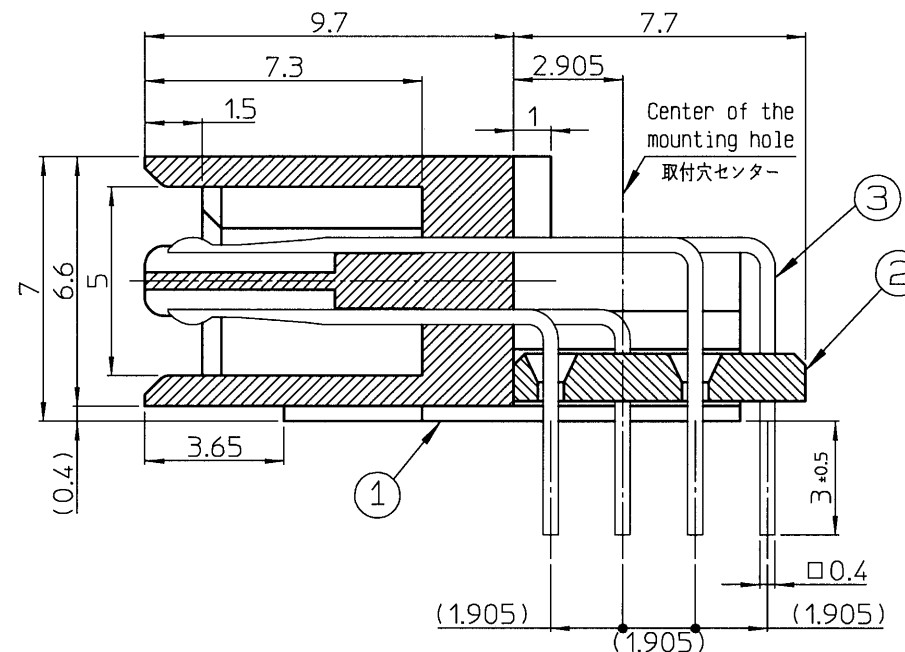
X-X' Cross-section(Scale 5:1)
