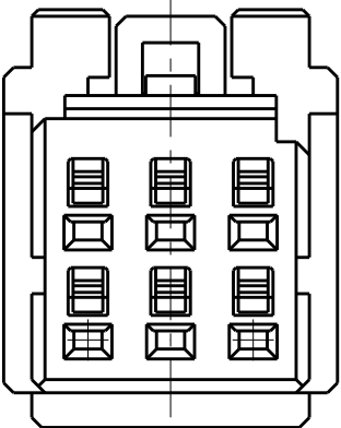
6POS(X-KEY): 9-1827864-3
