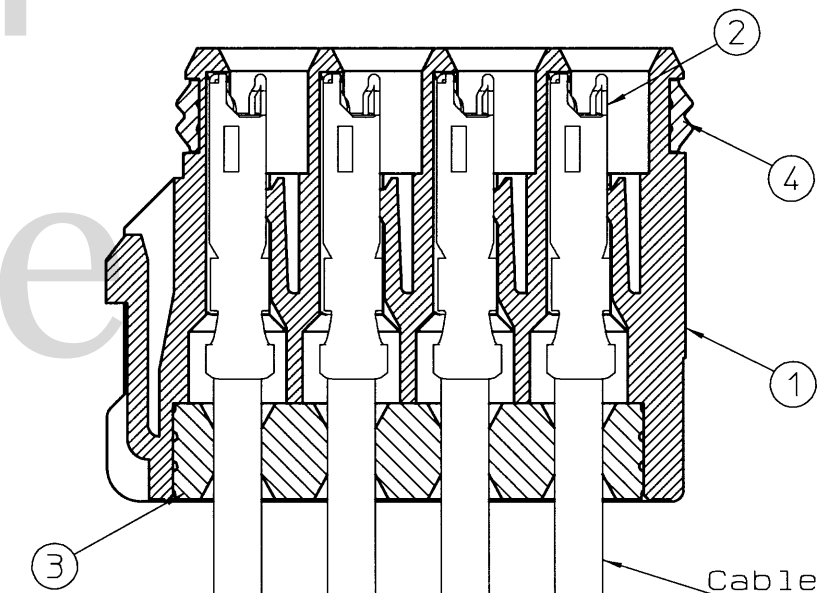
X-X' Cross Section (Contact Inserted) (3:1)
