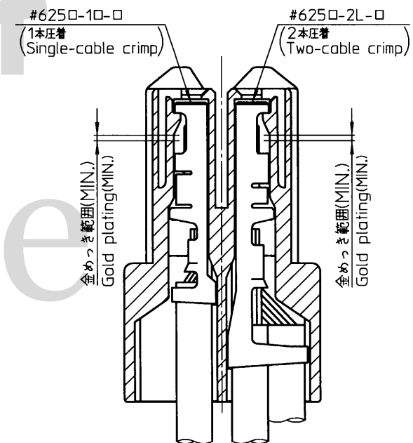
X-X'断面/Cross-section #625□-□□-□挿入時/Inserted
