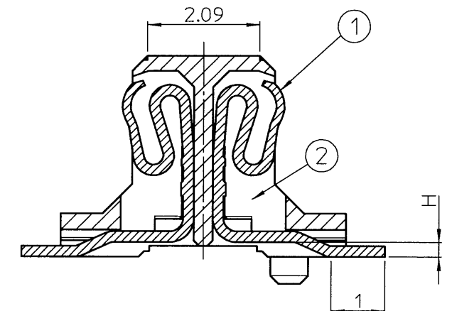
X-X' Cross-section(10:1)
