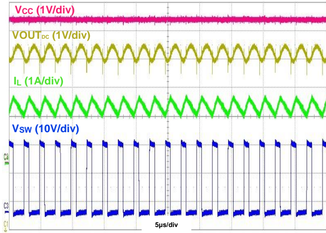
Figure 27. Steady State, Iout = 2A
