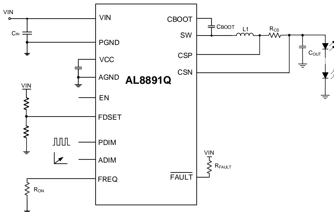
Figure 1. Typical Application
