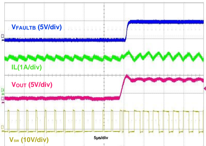
Figure 36. LED+ Short to LED- Recovery, VIN = 12V
