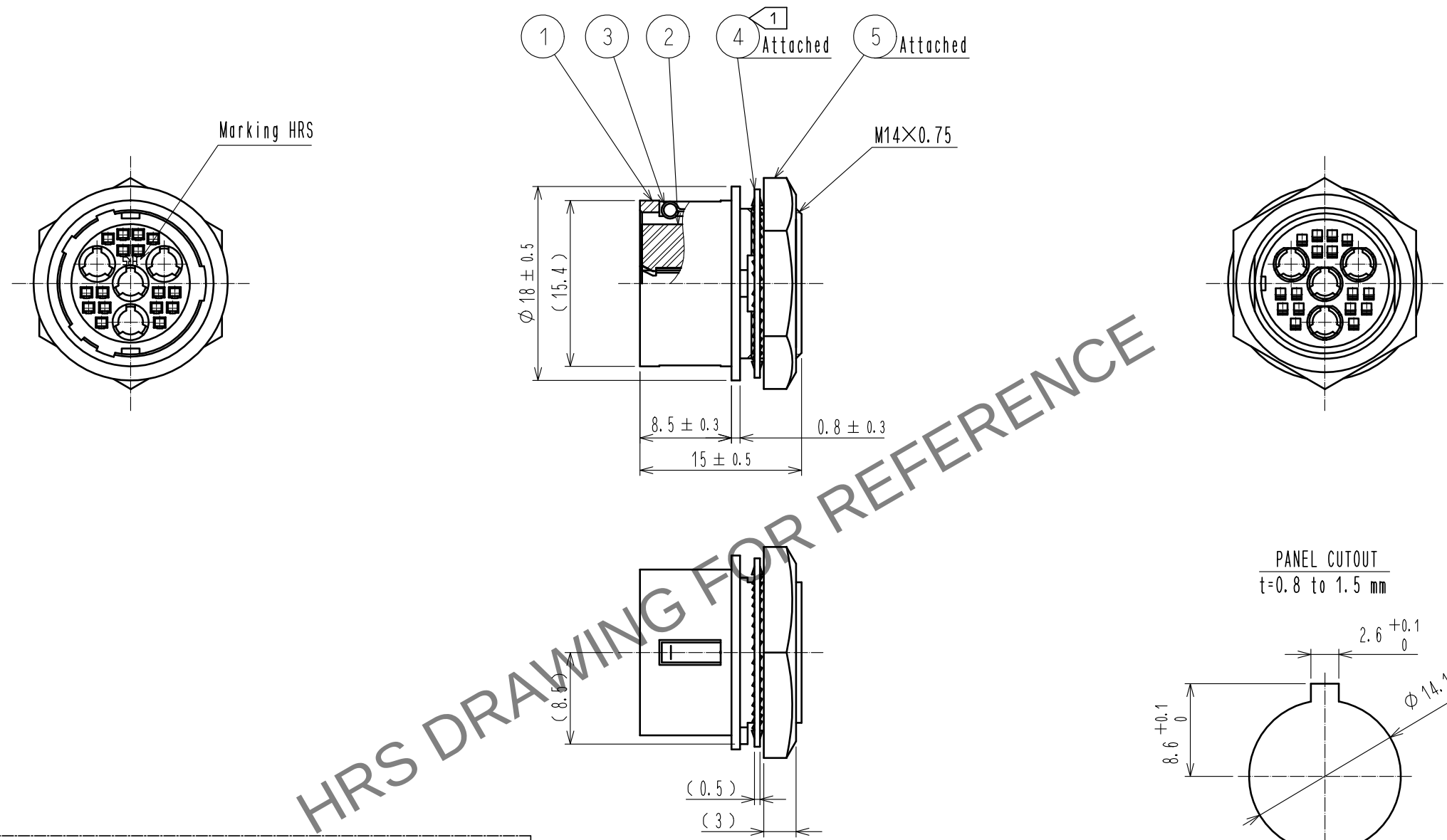
Harness drawing
