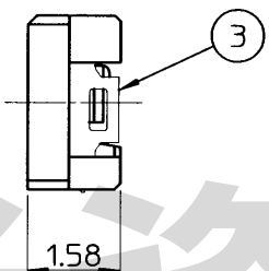
X-X' mated cross section(20:1) USLS00-40-X/USLS20-40
